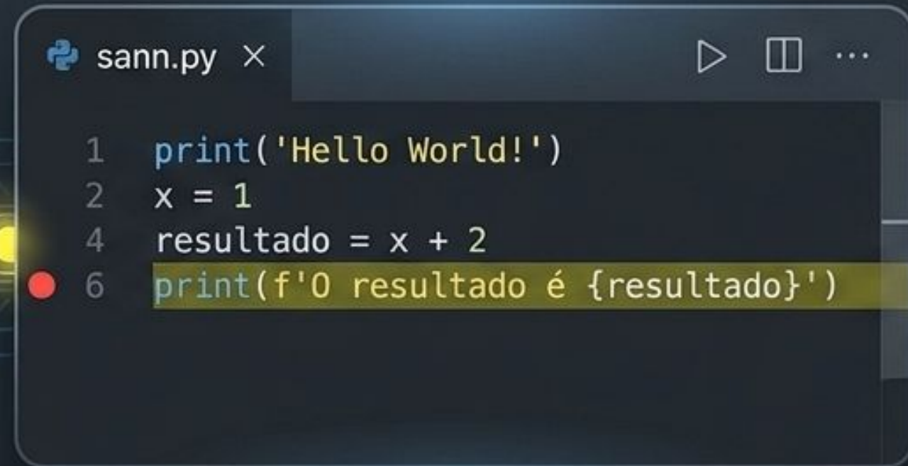
The Code
